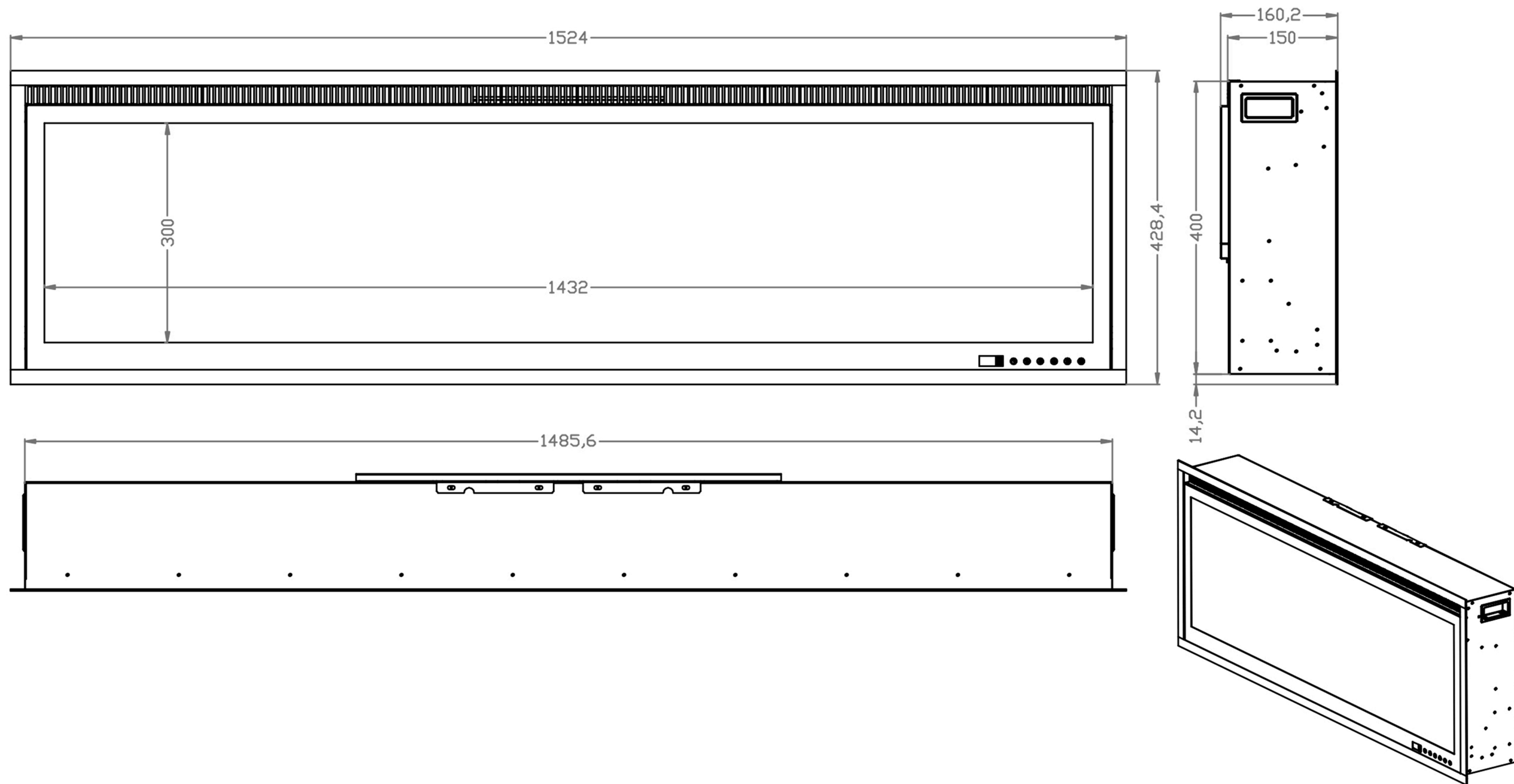
Glow Fire Smart Wall 60
