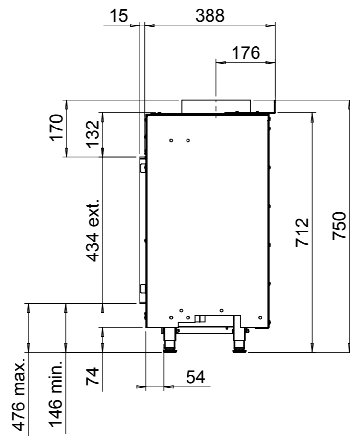
Dimensional drawing Relaxed Premium L - cover strip large
