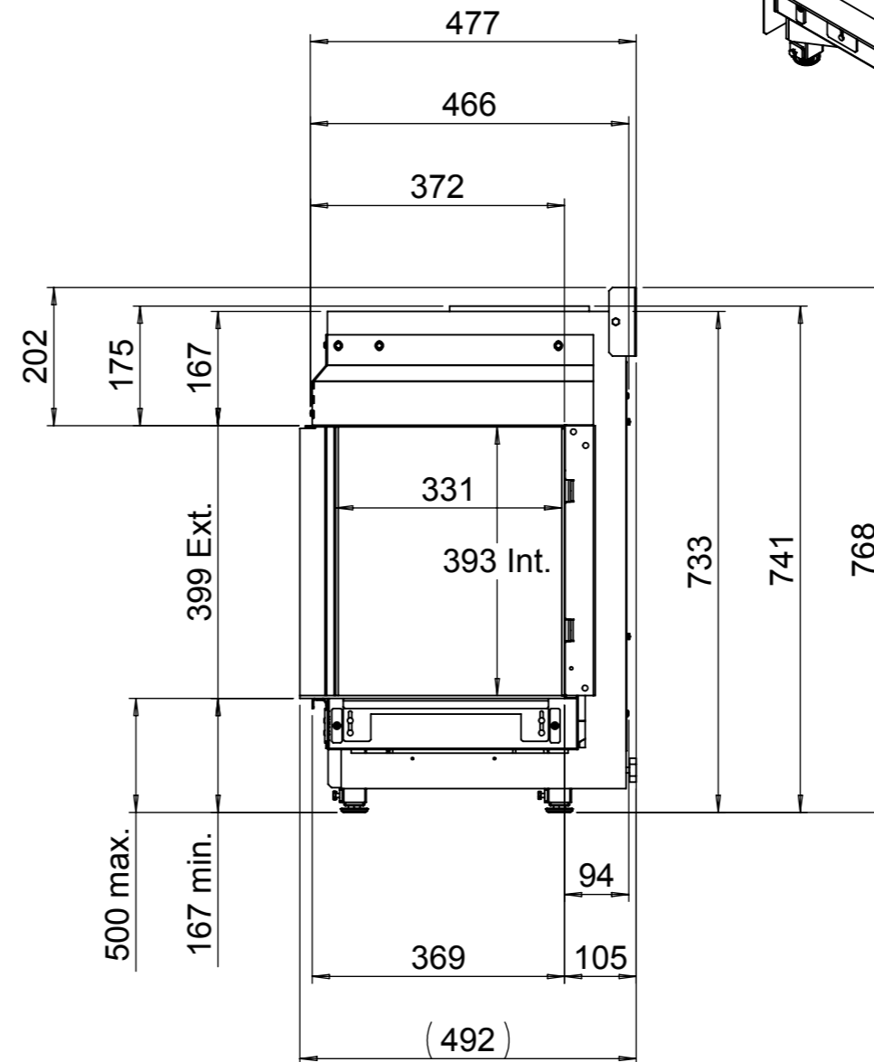
Dimensional drawing Duet Premium L right - cover strip large
